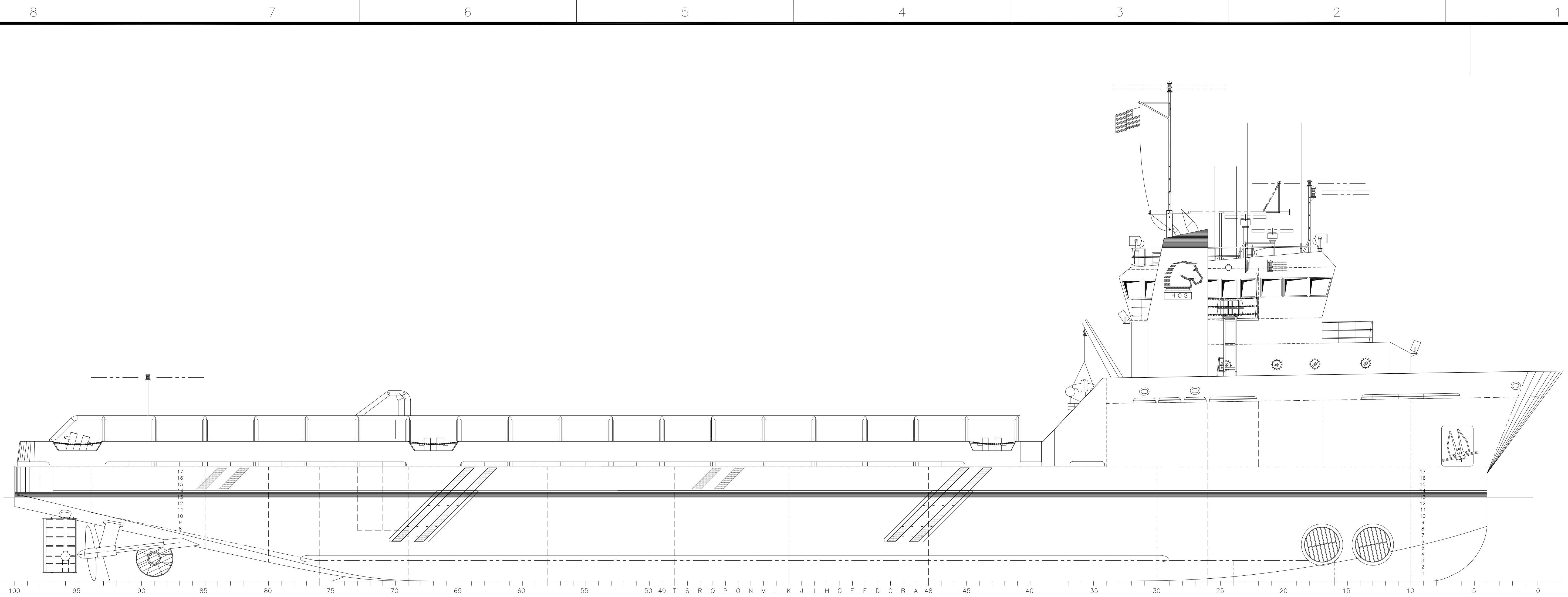
OUTBOARD PROFILE
