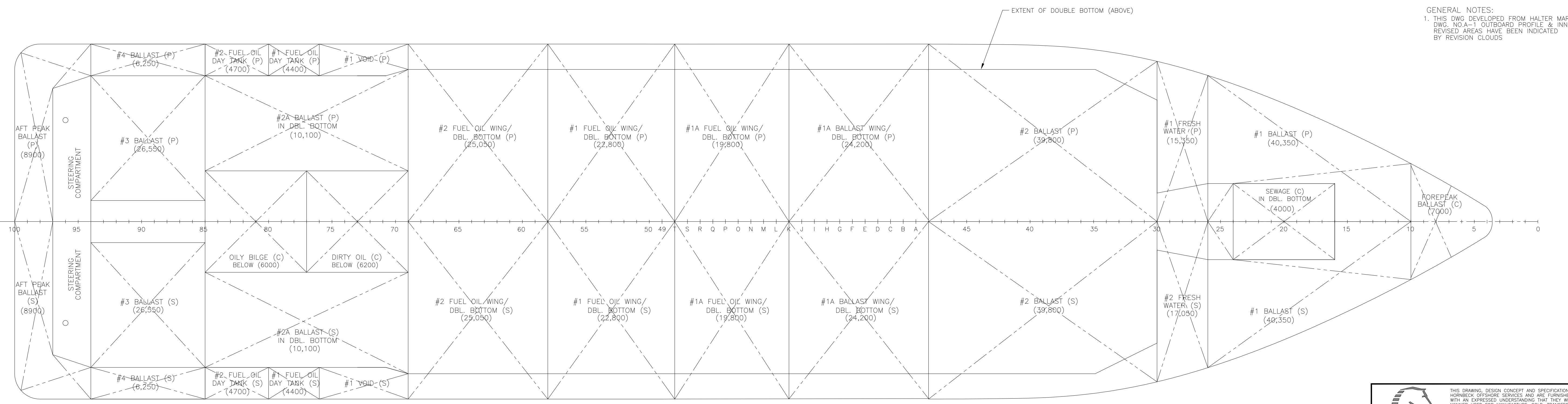
DOUBLE BOTTOM PLAN
