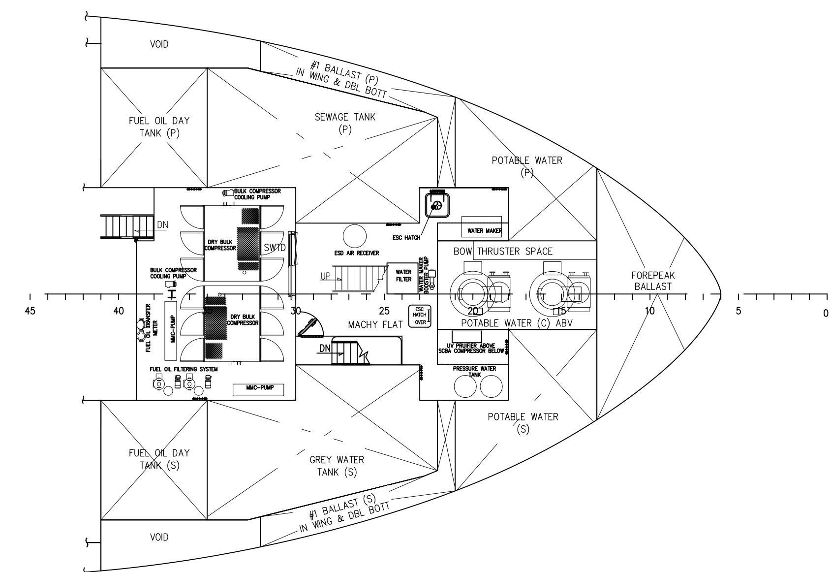
MEZZANINE FLAT
