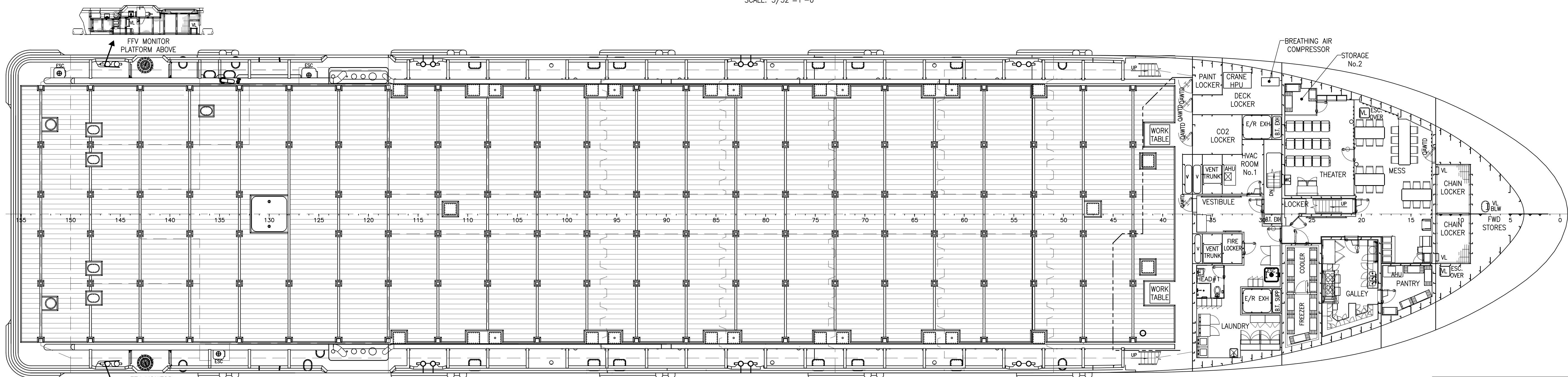
MAIN DECK
