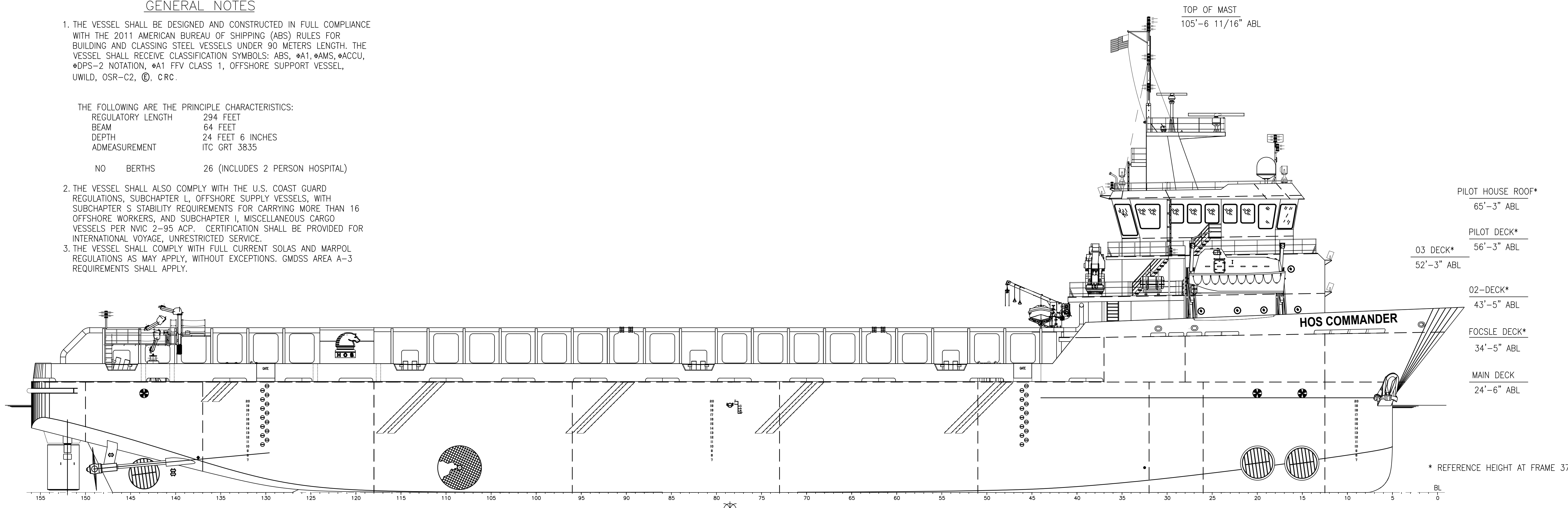
OUTBOARD PROFILE
