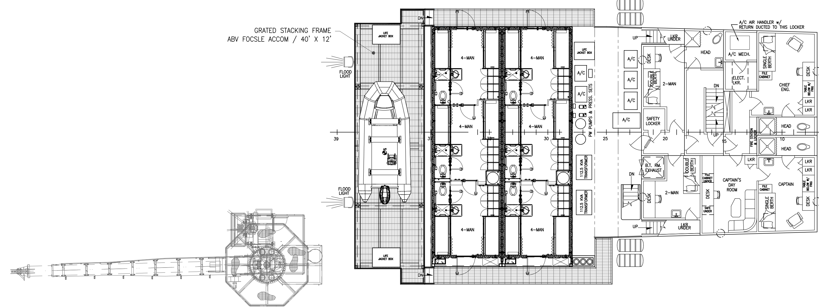
01 DECK 35'-6" ABOVE BASELINE
