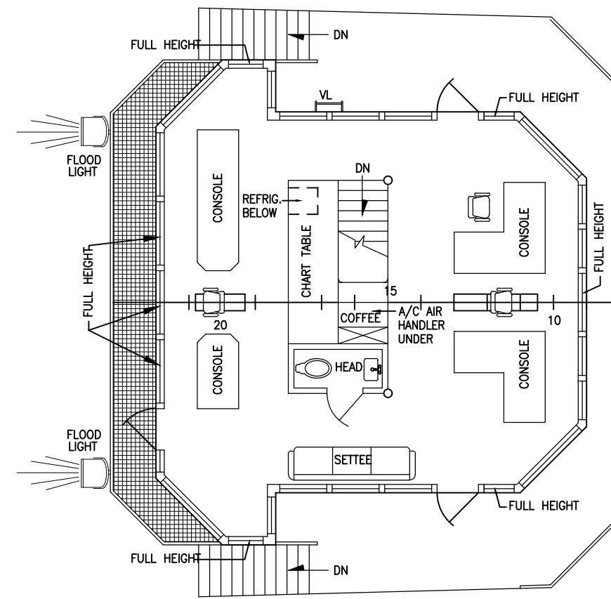
BRIDGE DECK 45'-0" ABOVE BASELINE
