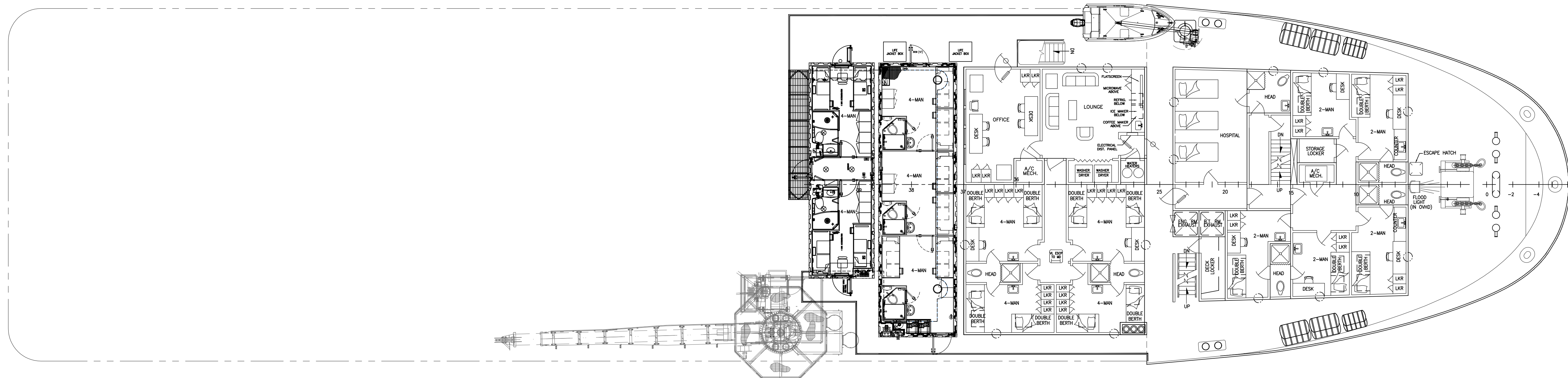
FOCSLE DECK 26'-0" ABOVE BASELINE
